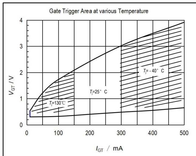
Fig10. Gate Trigger Area at various Temperature
